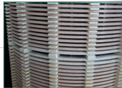
disc winding
