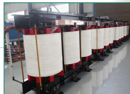
layer winding
